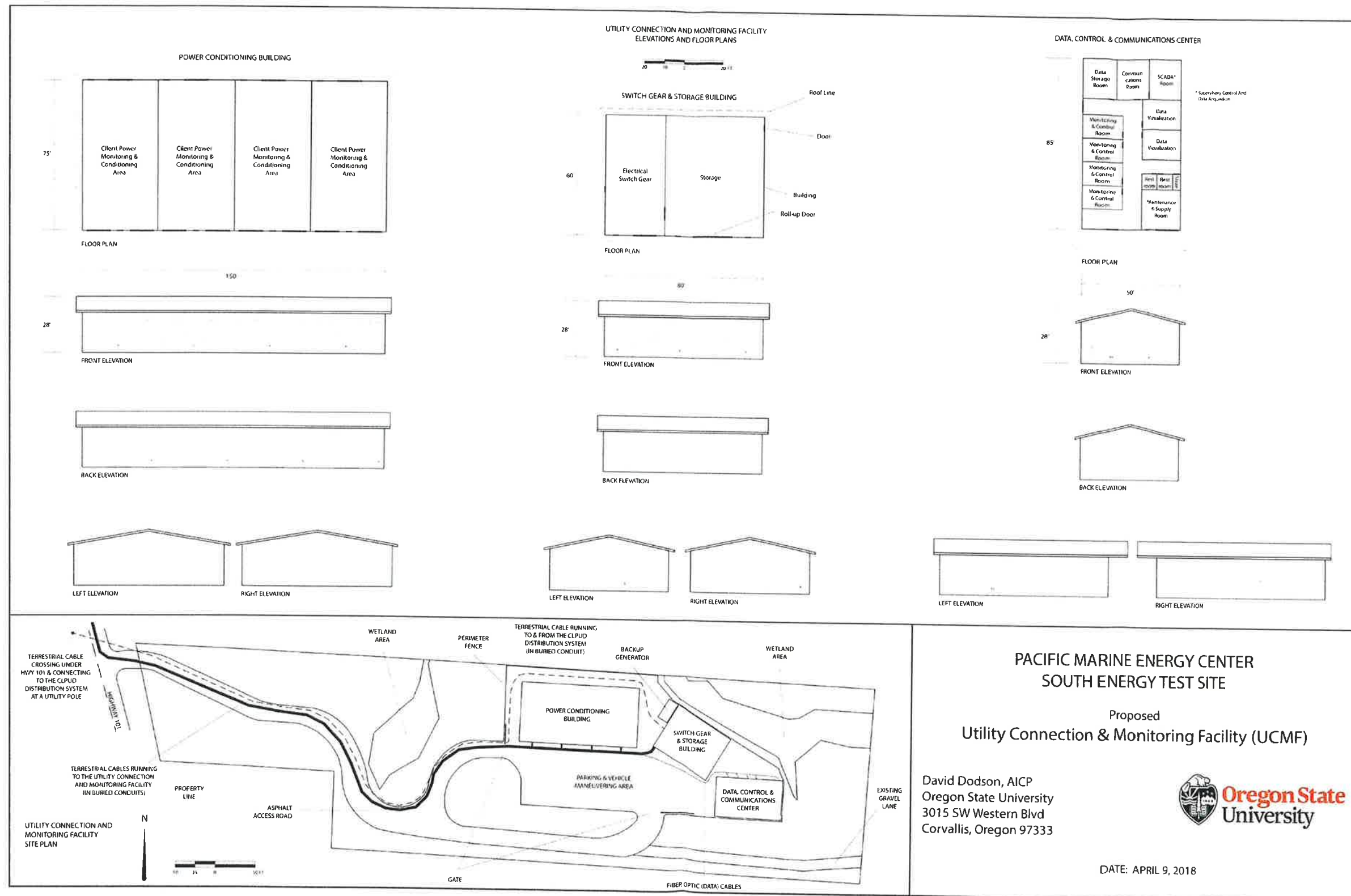
Proposed PMEC-SETS Utility Connection and Monitoring Facility site plan and elevations.
